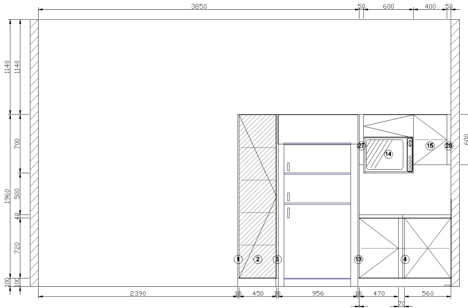
A View elevation drawing
