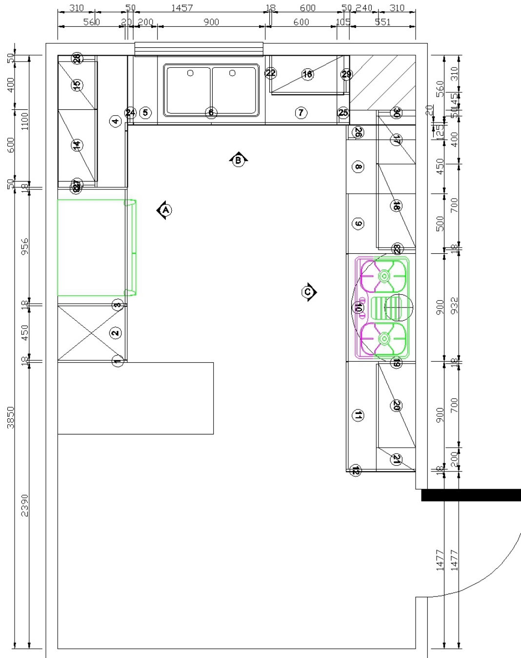
Plan drawing
