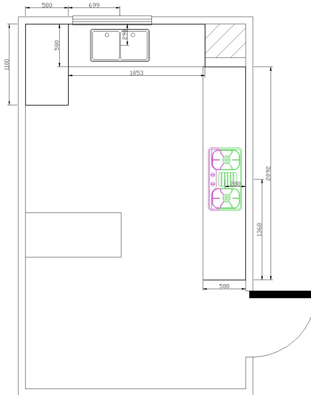
Worktop plan drawing
